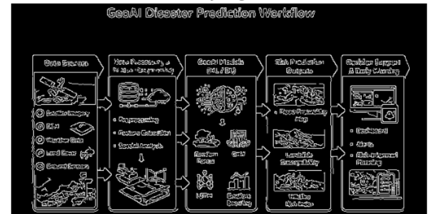
Canny Edges
